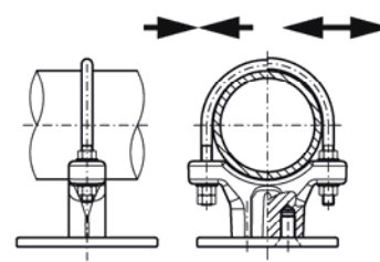
loose / fixed bearing F5/L5
