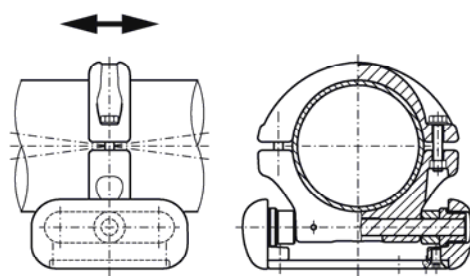
loose roller bearing L1
