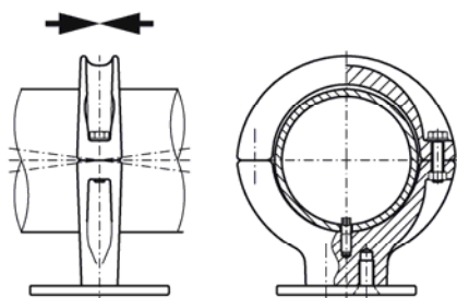
fixed metal on metal bearing F3
