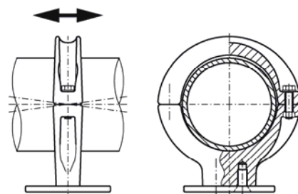
loose metal on metal bearing L3
